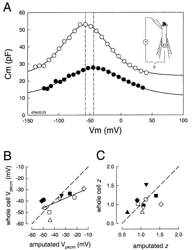
Fig. 1 A Membrane capacitance of outer hair cells (OHCs) before (open circles) and after (closed circles) electrical amputation in a microchamber. Parallel dashed lines indicate V_{\text{pkcm}} for each trace. B Comparison of V_{\text{pkcm}} for whole cell and amputated regions for 10 cells. Dashed diagonal line indicates equality. Solid line is linear fit to data. C z values for the same 10 cells. Note variability in whole cell z value
